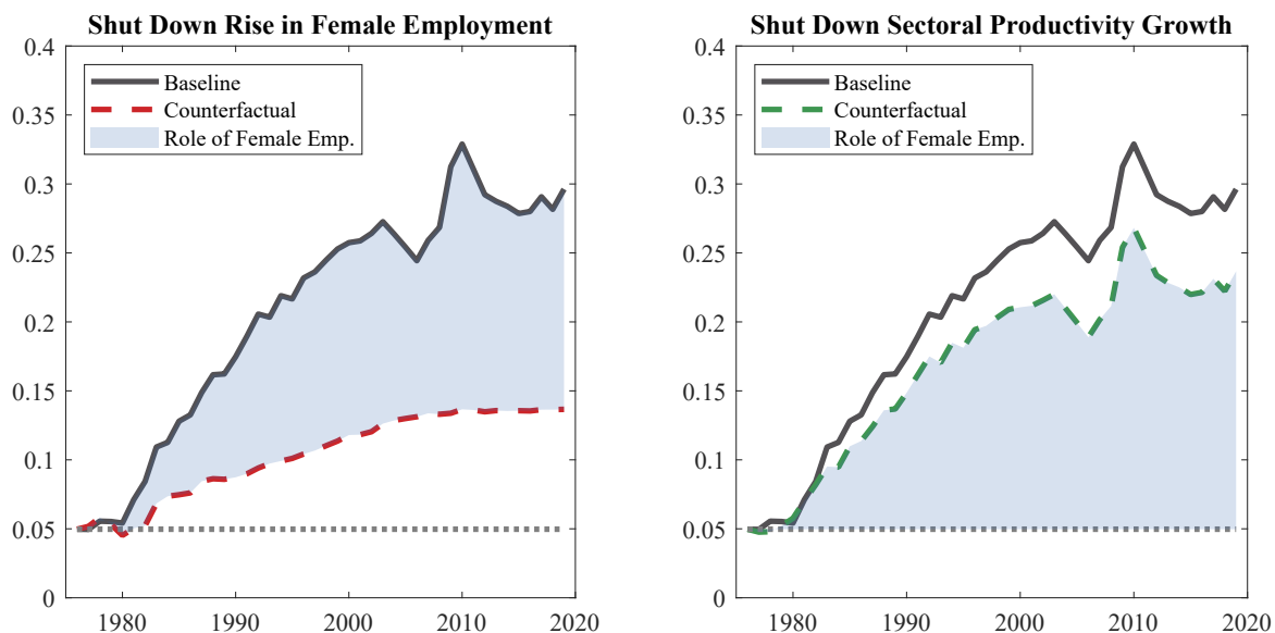
Figure 8: Counterfactual Analysis
