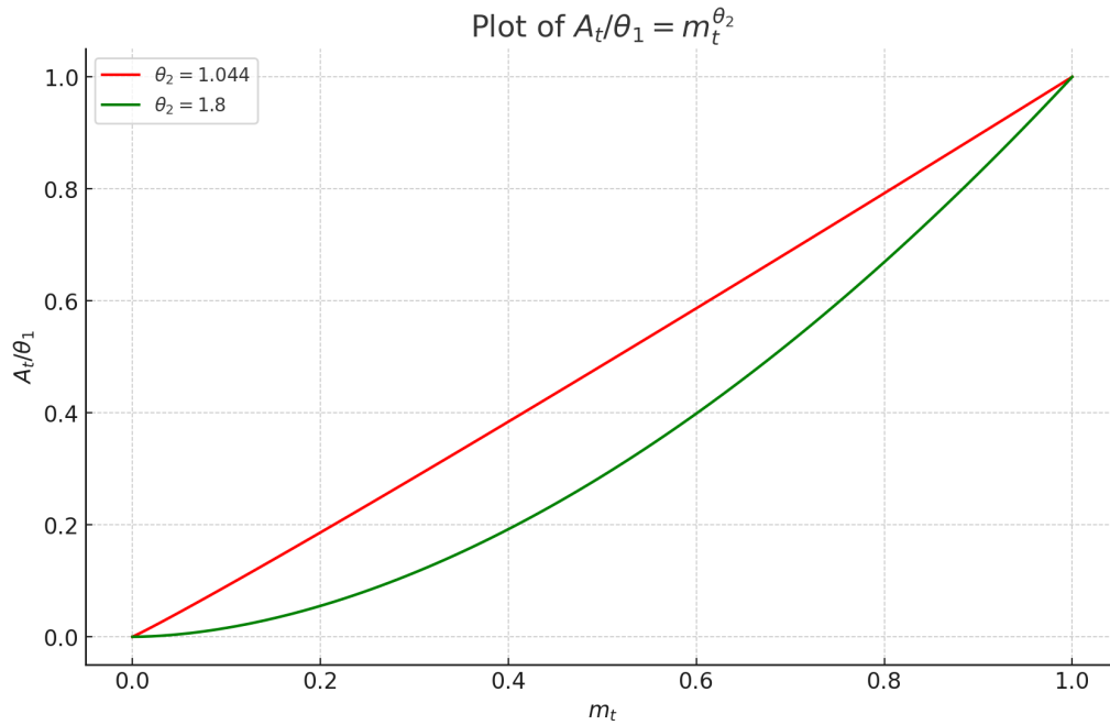
Figure 11: Normalized abatement cost function for different convexity of the curve. The red (green) curve represents the benchmark assumption for the public (private) sector.
