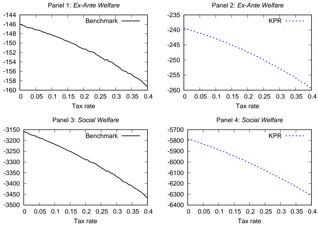
Figure 6: Ex-ante Welfare and Social Welfare responses to changes in the capital tax rate. Benchmark model (solid lines) and KPR specifications (dashed lines).
