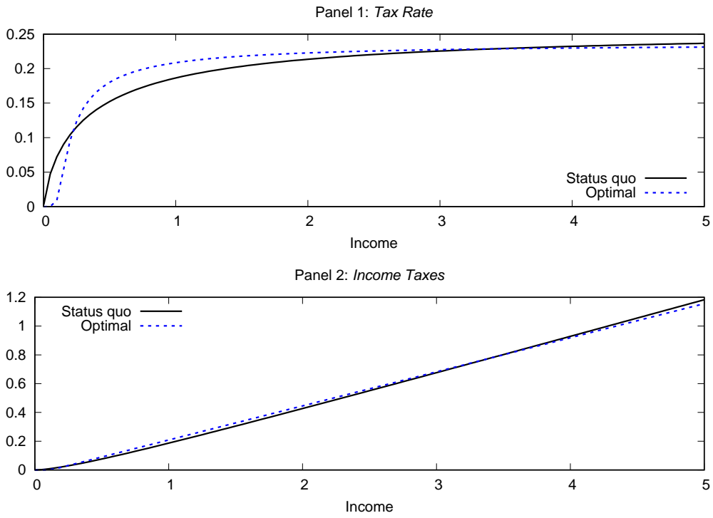
Figure 7: Tax Functions with a fixed G . Status quo Gouveia/Strauss Estimates Vs. Optimal Schedule (dashed).
