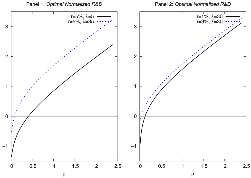
Figure 1: Optimal entrepreneurs' choices on R&D investment. The optimal \rho^* corresponds to the root of these functions.
