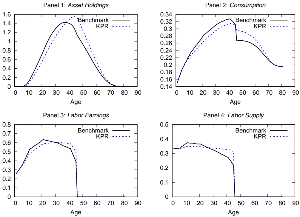
Figure 3: Average Cross Sectional profiles of Asset Holdings, Consumption, Labor Earnings, and Hours Worked. Benchmark model (solid line) and KPR preference specifications (dashed line).
