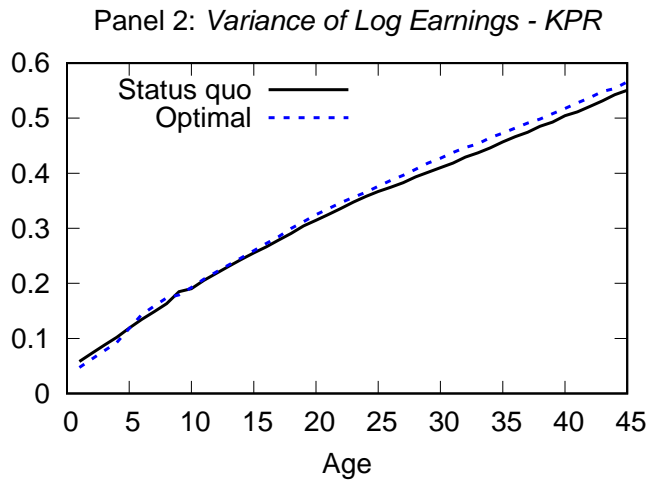
Figure 4: Pre-tax Labor Earnings Inequality. The status quo stands for the pre-reform equilibrium (solid line). The other profiles (dashed lines) are computed under the optimal taxation scheme with either assumption on preferences.
