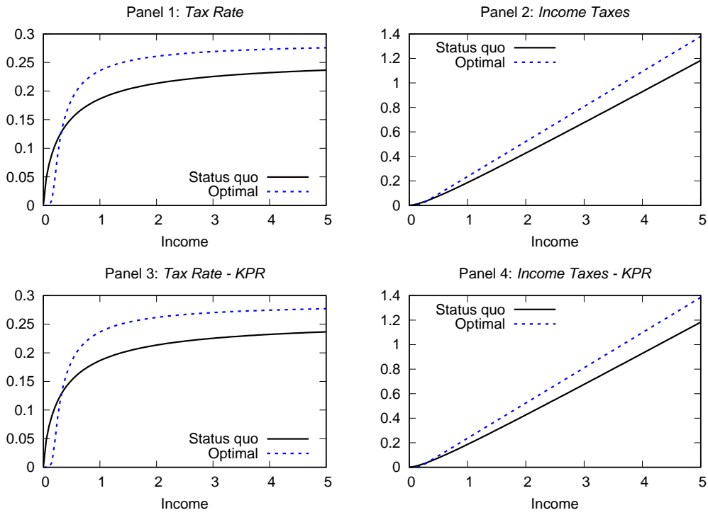
Figure 8: Income Tax Functions with a fixed G/Y ratio. Status quo Gouveia/Strauss Estimates Vs. Optimal Schedule (dashed).
