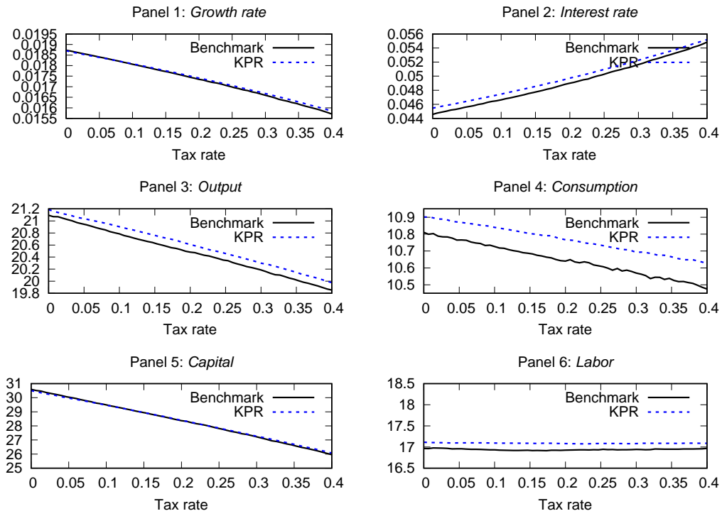
Figure 9: Growth Rate, Interest Rate, Output, Capital, Consumption and Labor equilibrium responses to changes in the capital tax rate. Benchmark model and KPR specifications (dashed).
