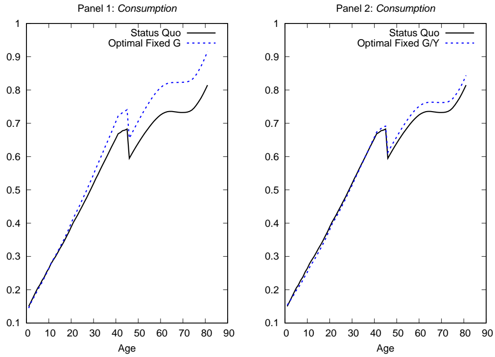
Figure 5: Average Life-cycle profiles of Consumption. The status quo stands for the pre-reform equilibrium (solid line). The other profiles (dashed lines) are computed under the optimal taxation scheme with either a fixed G or fixed G/Y .
