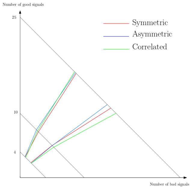
Figure 7a: Full Sample IC - Belief Updating
