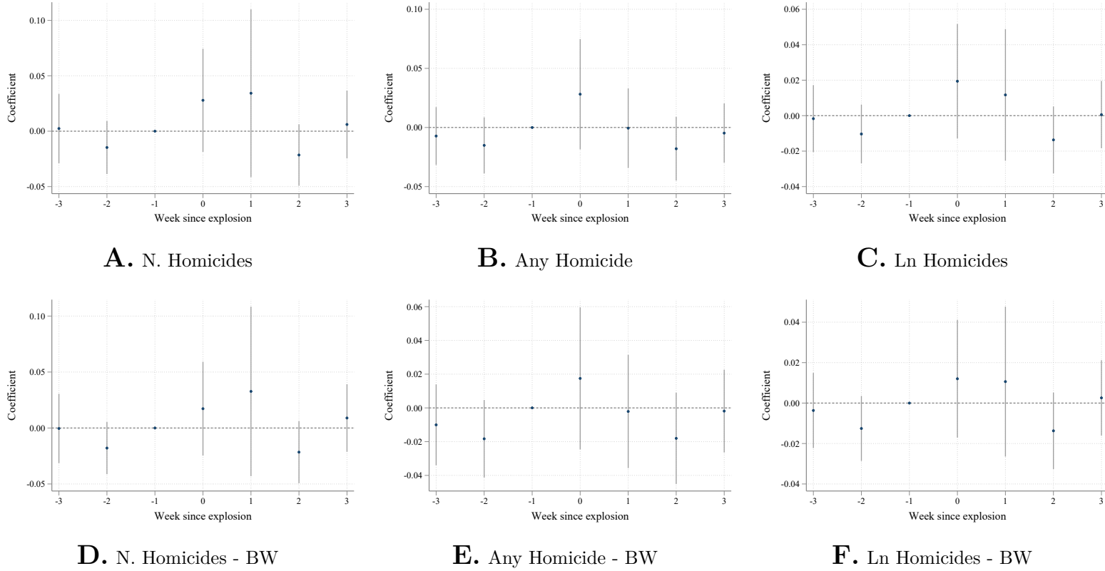
FIGURE A7. Homicides and Landmine Explosions: TWFE
