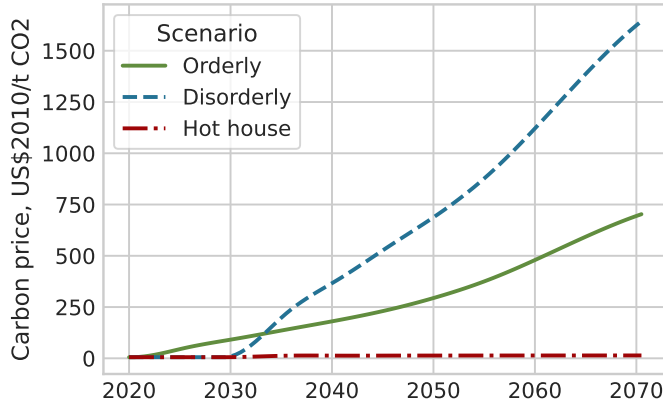
FIGURE 5: Carbon tax level trajectories from NGFS scenarios.
