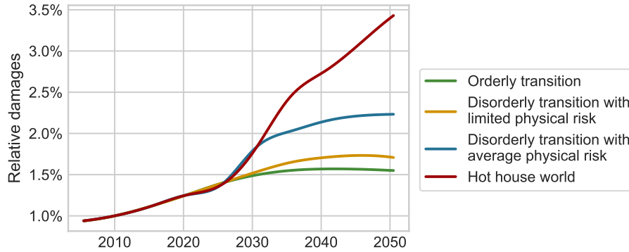
FIGURE 8: Physical risk trajectories across scenarios.
