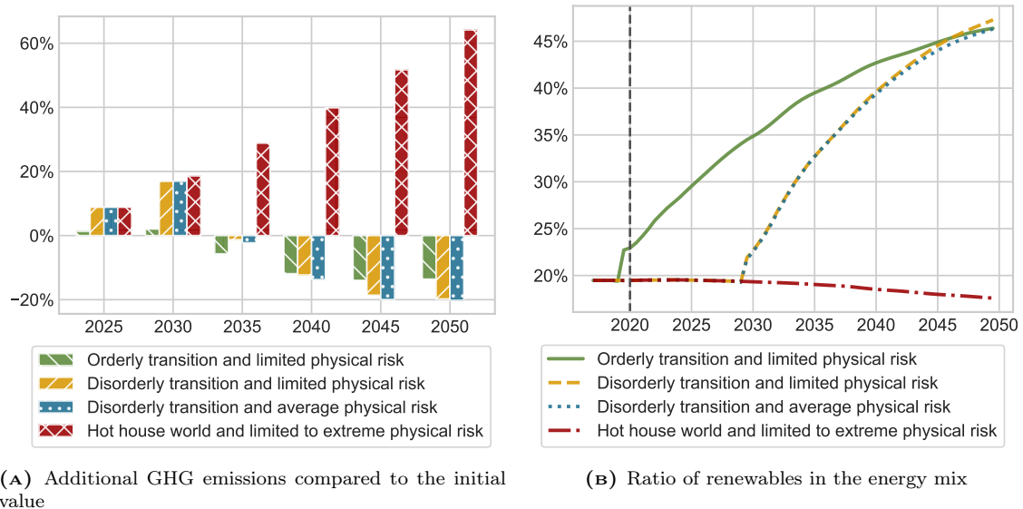
FIGURE 11: Transition results for GHG emissions and energy mix across NGFS scenarios.
