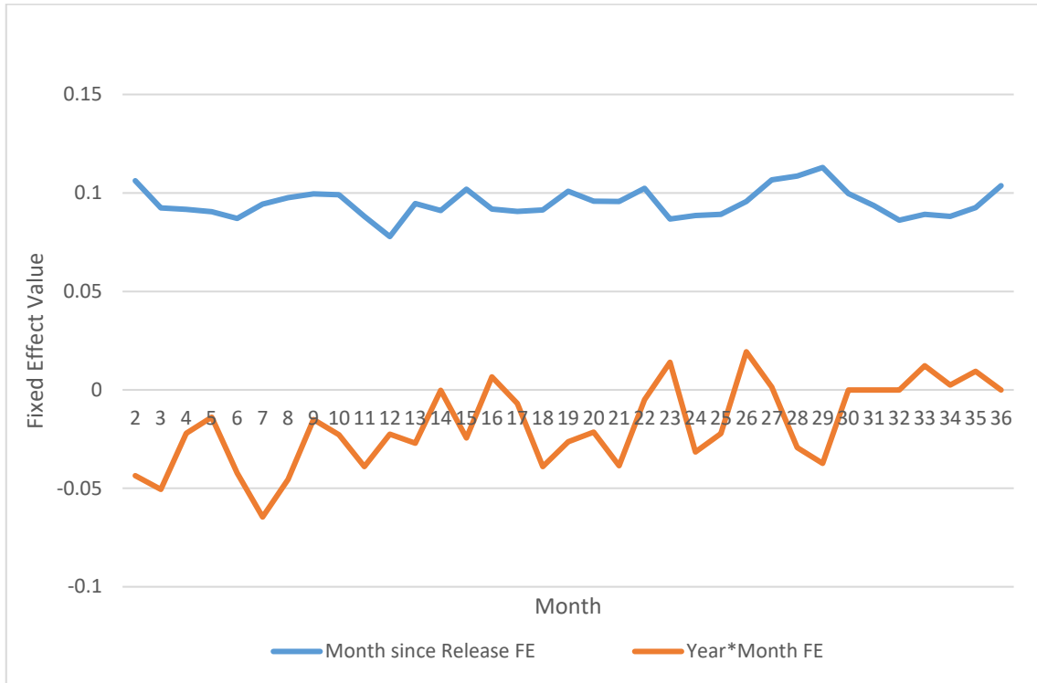
Figure 6. Month*Year FE and Month since Release FE
