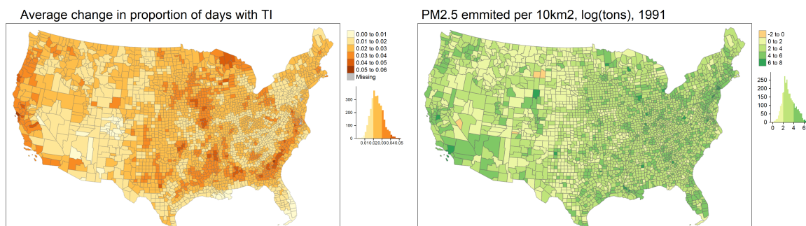
Figure 4: Identifying variation of the thermal inversion instrument.
