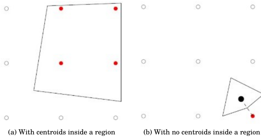
Figure 14: Imputation of raster values to counties (image from Dechezleprêtre et al. (2019) )
