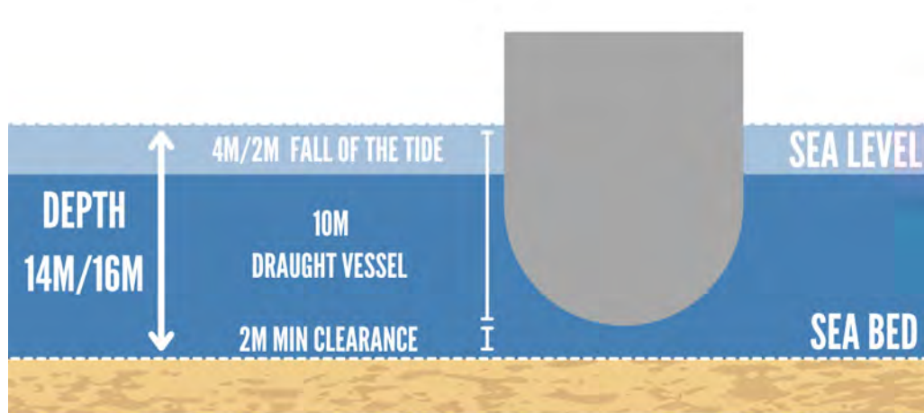
Figure A.4: Depth requirement for safe anchorage.
