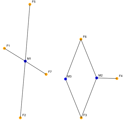
Figure 2: Fragmented school network
