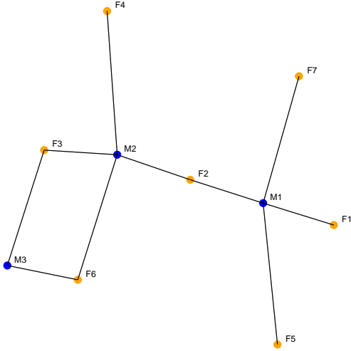
Figure 1: Complete school network
