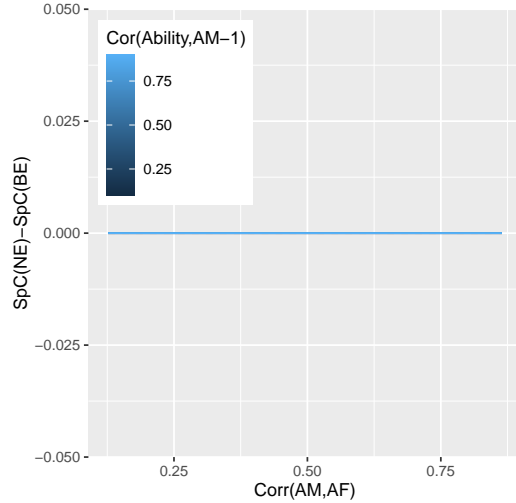
(c) Distribution of NE VA for different level of \text{corr}(A_M, A_F) and BE VA for level of \text{corr}(A_{M,t}, A_{M,t-1}) and NE VA for \text{corr}(A_{M,t}, A_{M,t-1})=0.8
