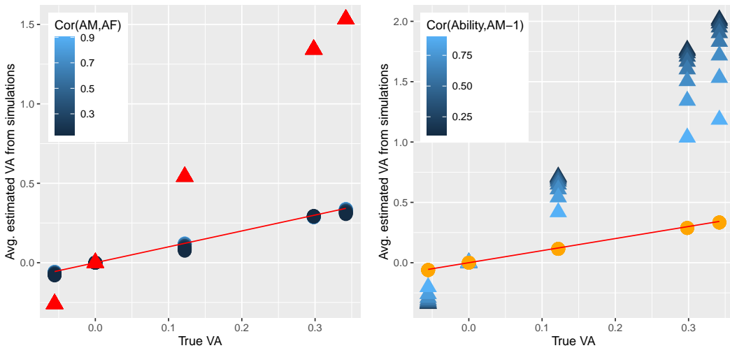
(c) Distribution of NE VA for different level of \text{corr}(A_M, A_F) and BE VA for level of \text{corr}(A_{M,t}, A_{M,t-1}) and NE VA for \text{corr}(A_{M,t}, A_{M,t-1})=0.8 (d) Distribution of BE VA for different level of \text{corr}(A_{M,t}, A_{M,t-1}) and NE VA for \text{corr}(A_M, A_F)=0.58
