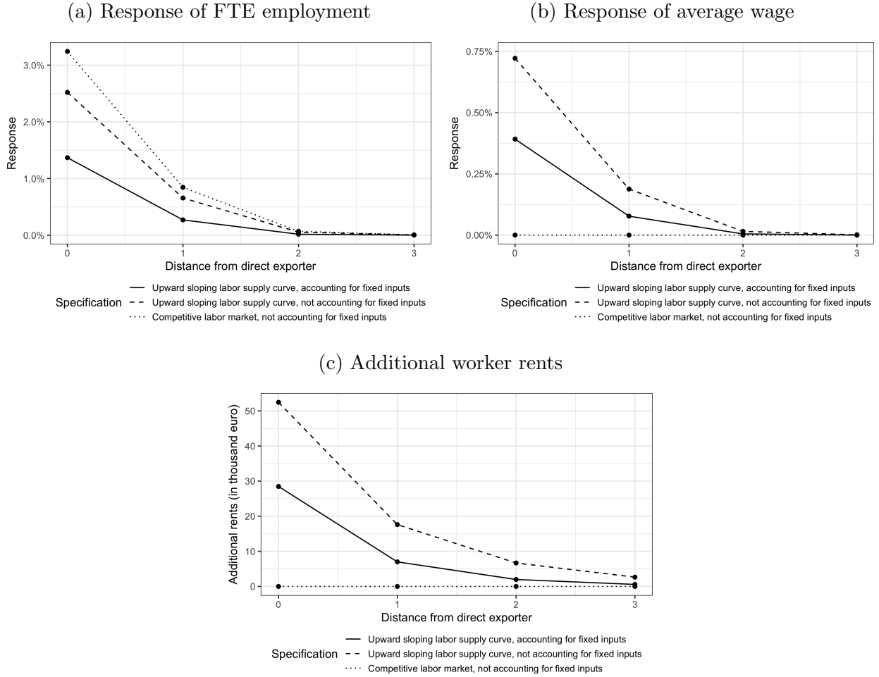
Figure 4: Simulation results of foreign demand shock transmission along the supply chain
