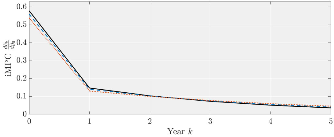
Figure 19: Intertemporal MPCs
