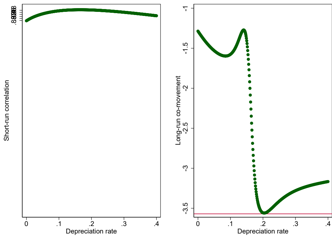
FIGURE A.8: Sensitivity analysis of the PIM-based series to a value of the depreciation rate ( \delta ) and a choice of initial year
