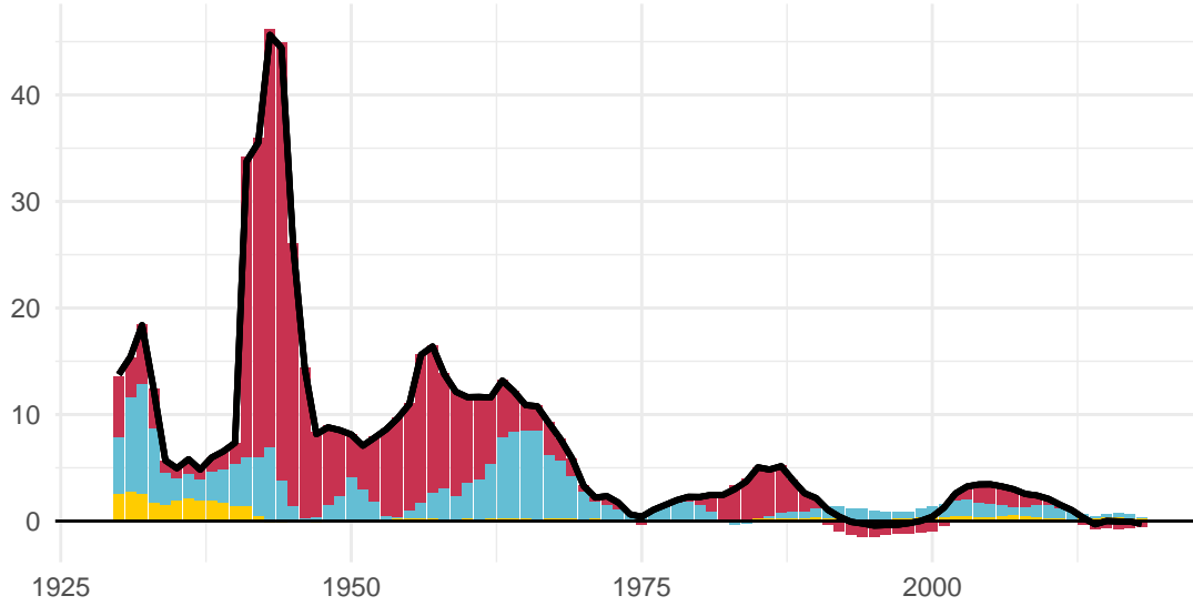
FIGURE A.11: Public R&D capital (annual growth rate) and its components
