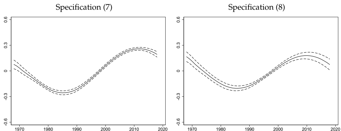
FIGURE 4: IDEA TFP BACKED OUT FROM THE IPF
