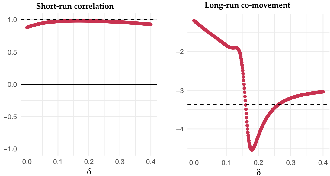
FIGURE A.9: Sensitivity analysis of the PIM-based series to a value of the depreciation rate ( \delta )
