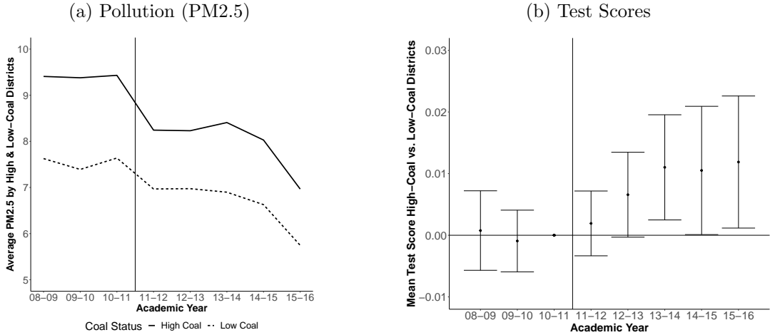
Figure 2: Difference-in-Differences
